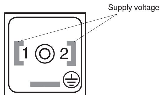
Connection diagram for plug form A (DIN EN 175301-803)
