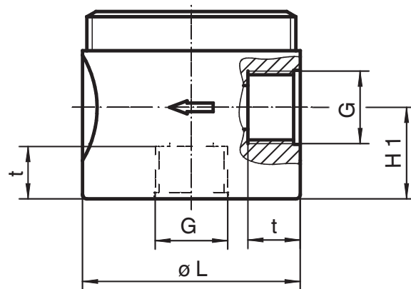
Angled body (code E)
