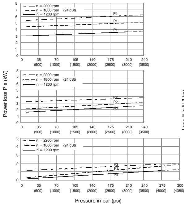
HYDROMECHANICAL POWER LOSS (TYPICAL)
