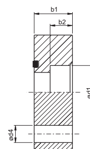
Socket weld
