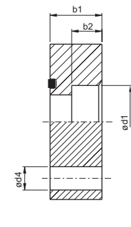
Socket weld
